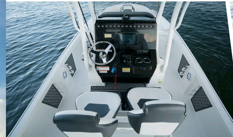
Helm center console, SST steering wheel, optional sport seats, and gunnel mount rod storage
